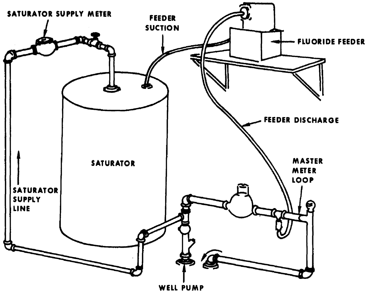
Figure 1. Pump Room
